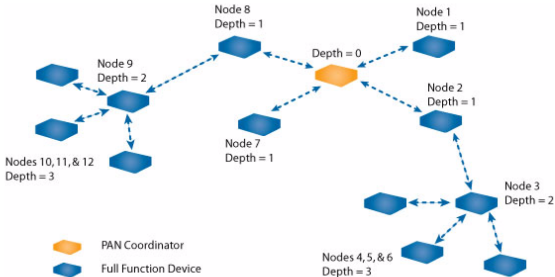
Figure 3: Network Depth
