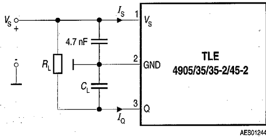
Unipolar Type TLE 4905
