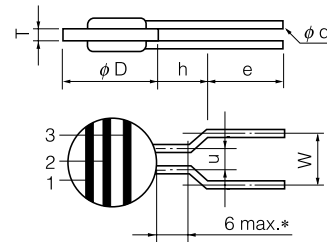
Crimped Lead Type Z Type
