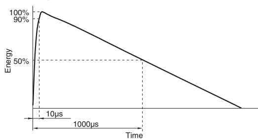
*2 10/1000μs test waveform
