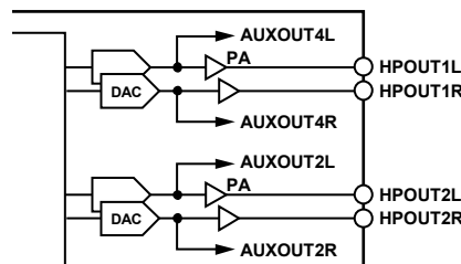
Figure 30. Headphone Outputs Section
