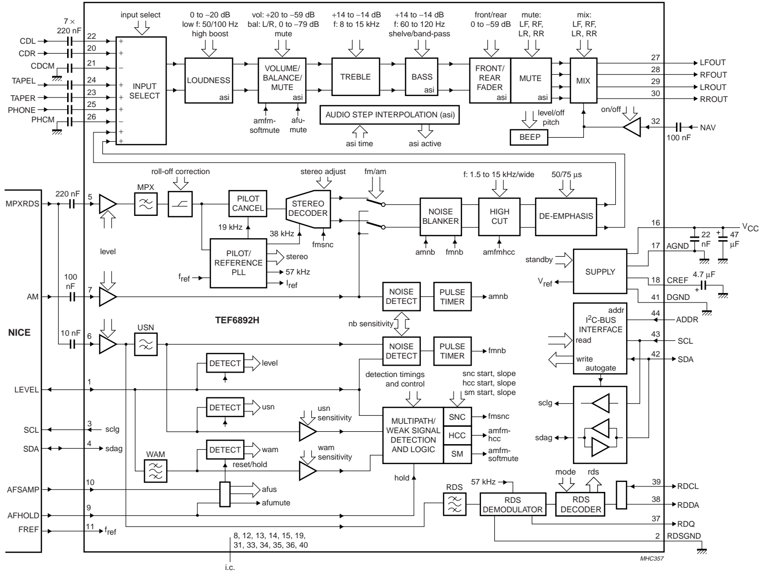
Fig.24 Application diagram.
