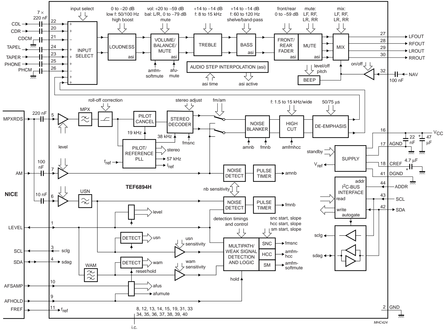
Fig.24 Application diagram.
