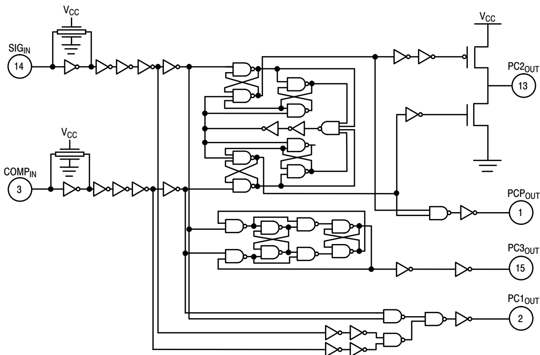
Figure 6. Logic Diagram for Phase Comparators
