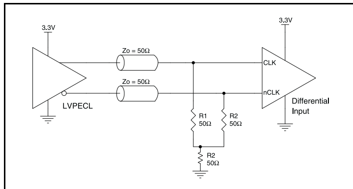
Figure 2D. CLK/nCLK Input Driven by a 3.3V LVPECL Driver
