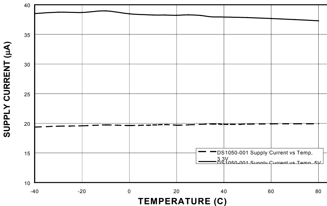
DS1050-001 SUPPLY CURRENT vs. TEMPERATURE
