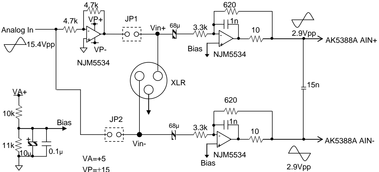
Figure 25.Input Buffer example1
