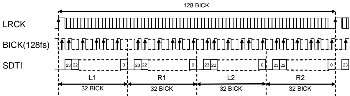
Figure 19. Mode 10 Timing
