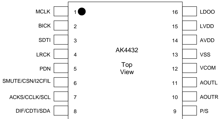
Figure 2. Pin Layout
