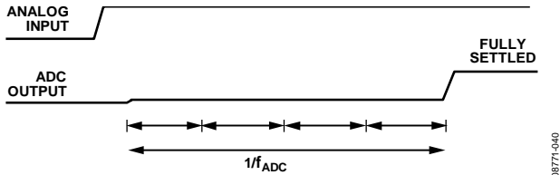
Figure 27. Sinc 4 Zero Latency Operation
