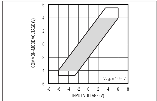
Figure 10. Common-Mode Voltage vs. Input Voltage (FSR = 2 \times V_{REF} )
