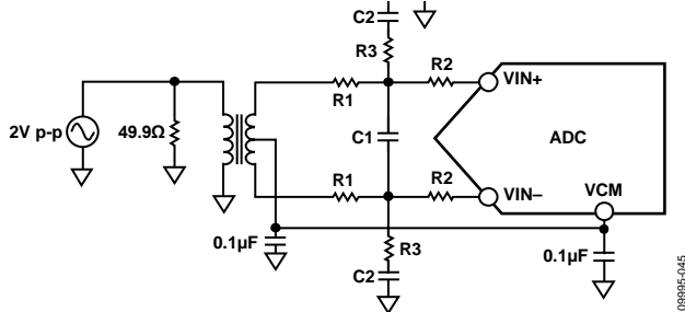
Figure 48. Differential Transformer-Coupled Configuration
