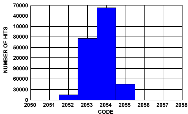
FIGURE 15. NOISE HISTOGRAM
