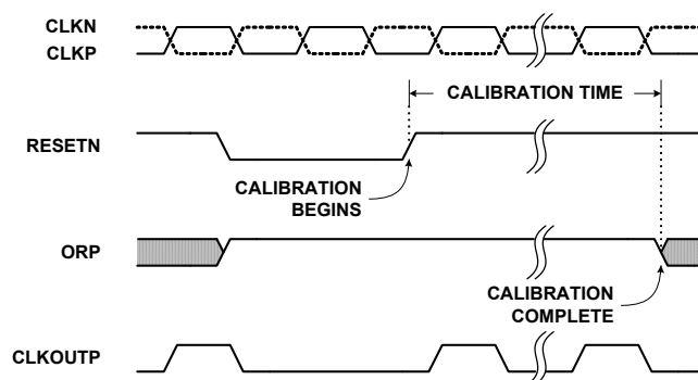
FIGURE 24. CALIBRATION TIMING
