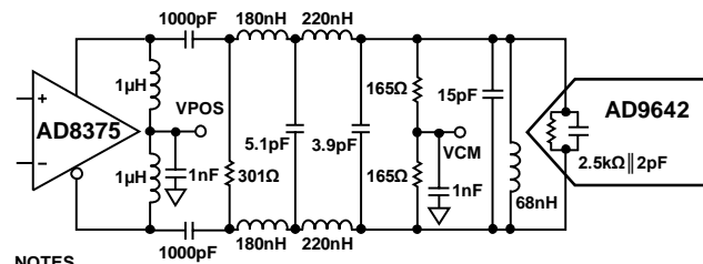
Figure 49. Differential Input Configuration Using the AD8375
