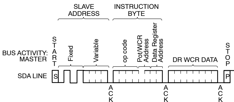
Figure 7. Write Timing
