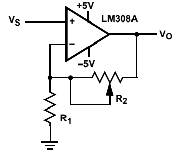
Noninverting Amplifier
