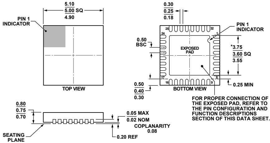
*COMPLIANT TO JEDEC STANDARDS MO-220-WHHD-5 WITH EXCEPTION TO EXPOSED PAD DIMENSION. Figure 54. 32-Lead Lead Frame Chip Scale Package [LFCSP_WQ] 5 mm × 5 mm Body, Very Very Thin Quad (CP-32-12) Dimensions shown in millimeters
